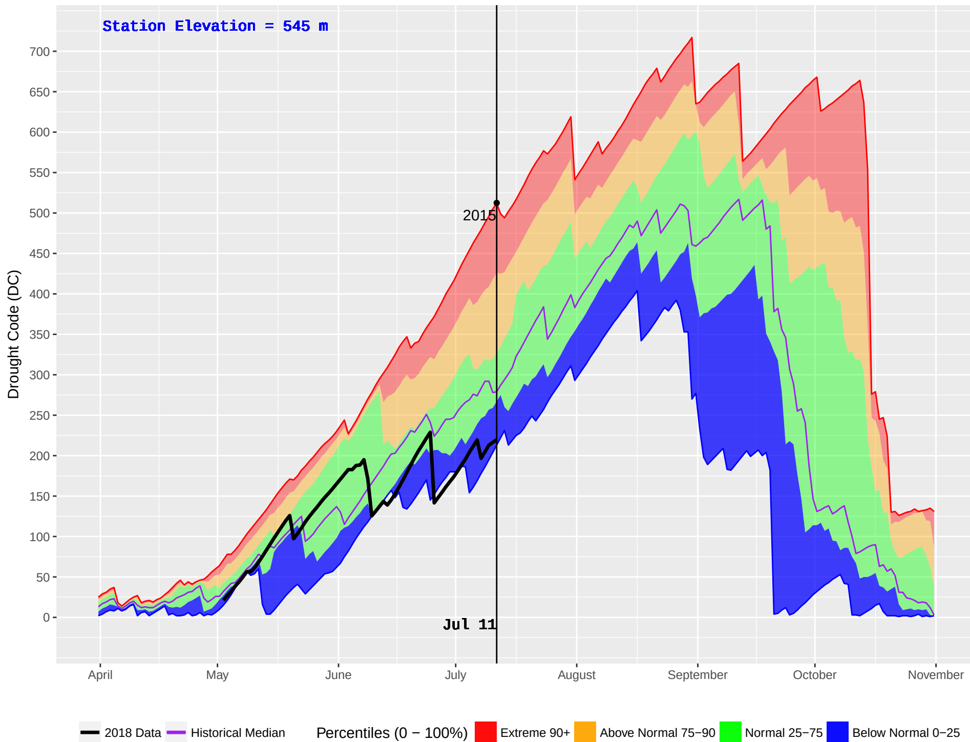
MEAGER CREEK (1083) : Historical (2010–2016) and Current (2018) Noon Drought Code (DC)
