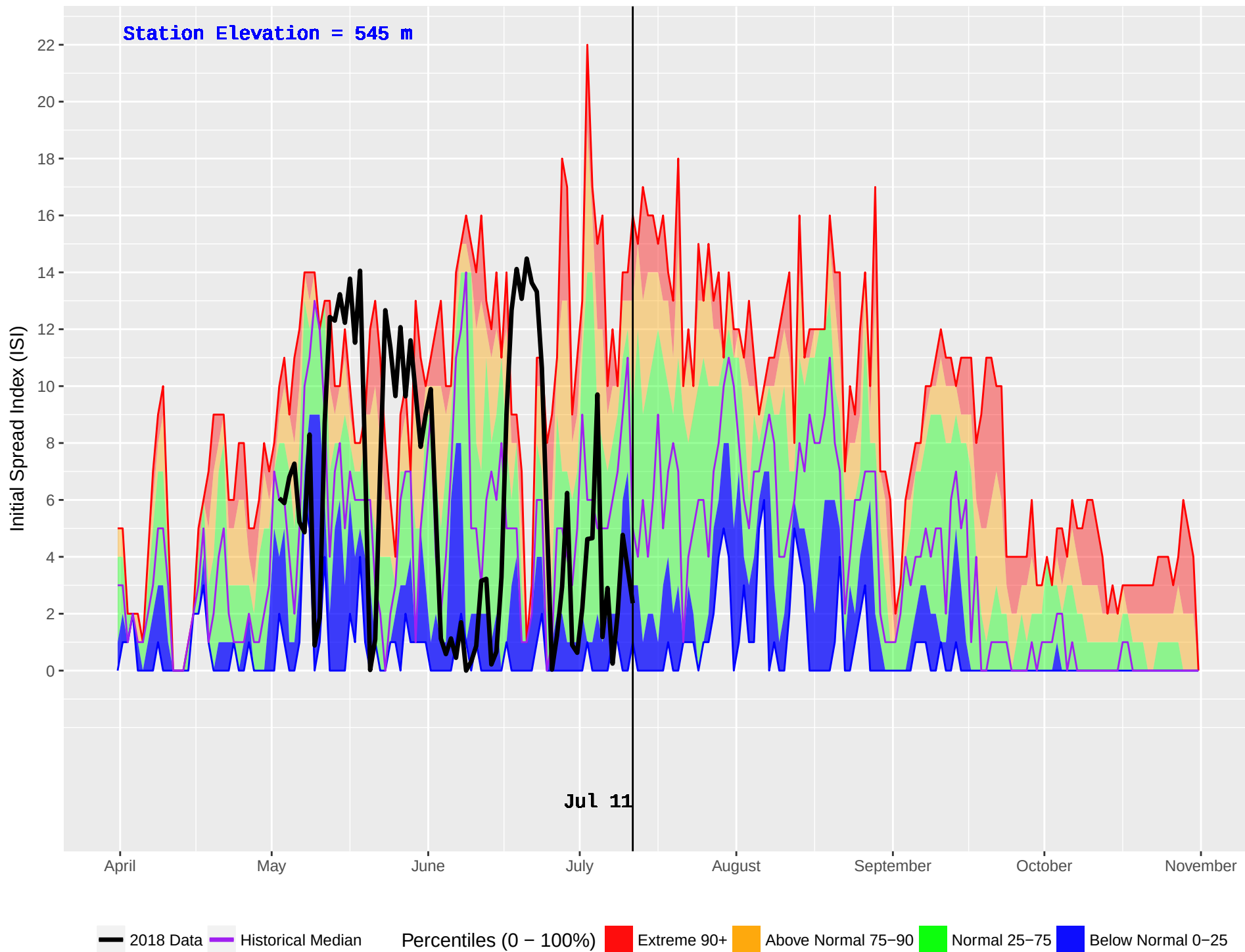
MEAGER CREEK (1083) : Historical (2010–2016) and Current (2018) Noon Initial Spread Index (ISI)
