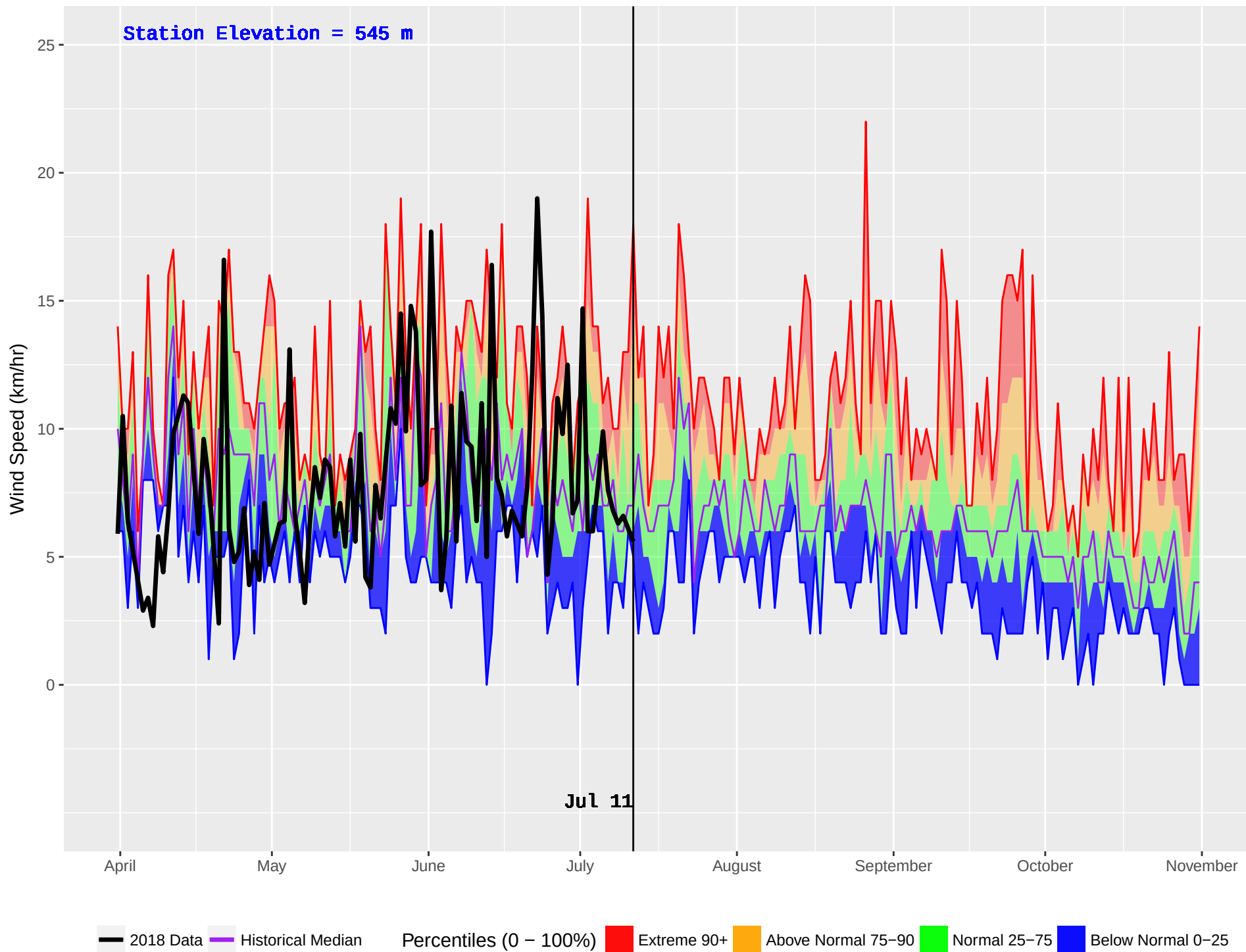
MEAGER CREEK (1083) : Historical (2010–2016) and Current (2018) Noon Wind Speed
