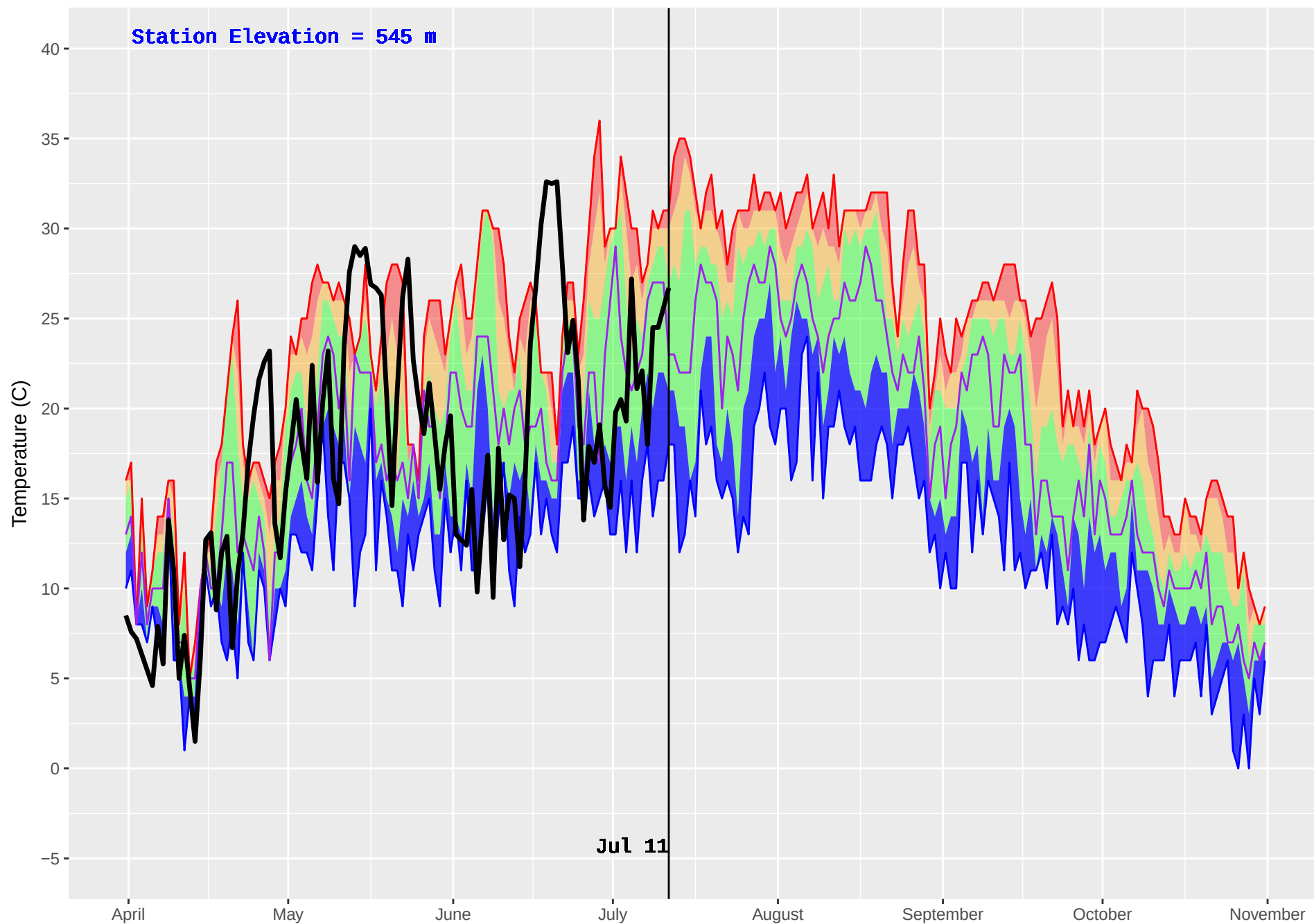
MEAGER CREEK (1083) : Historical (2010–2016) and Current (2018) Noon Temperature
